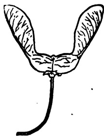
FIG. 245. — Fruit of Maple. (From Bailey.)
